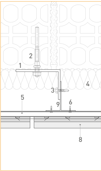
3. Horizontal detail
