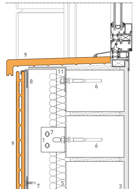
SILL - monoblock
