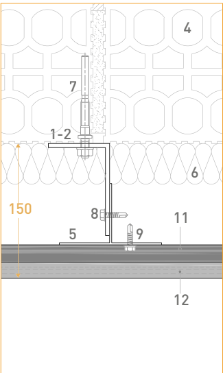
3. Horizontal detail
