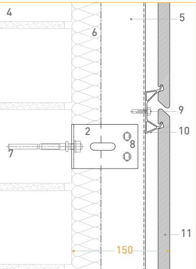
2. Stop bracket
