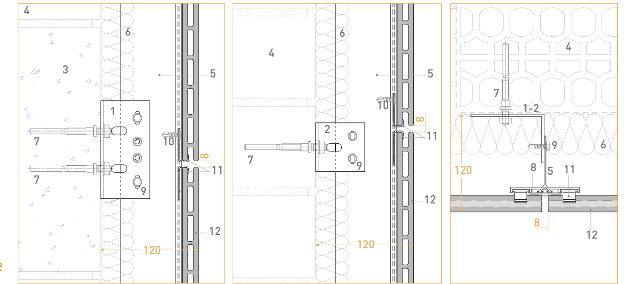
1. Support bracket
