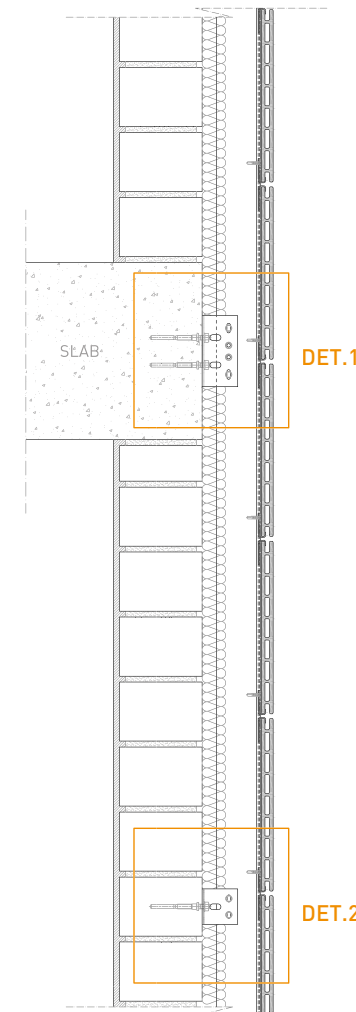
1. Support bracket
