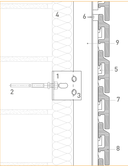
2. Stop bracket
